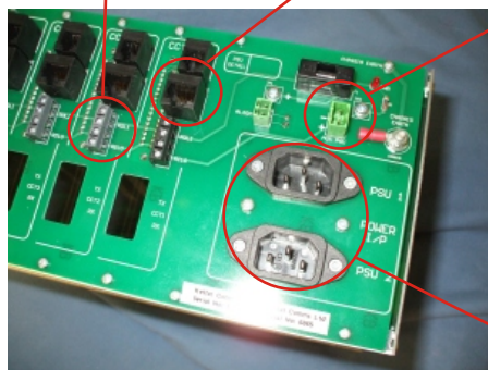
BACKPLANE VIEW
